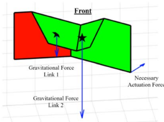
Figure 7: Geometrical Analysis of transFORM using MATLAB
